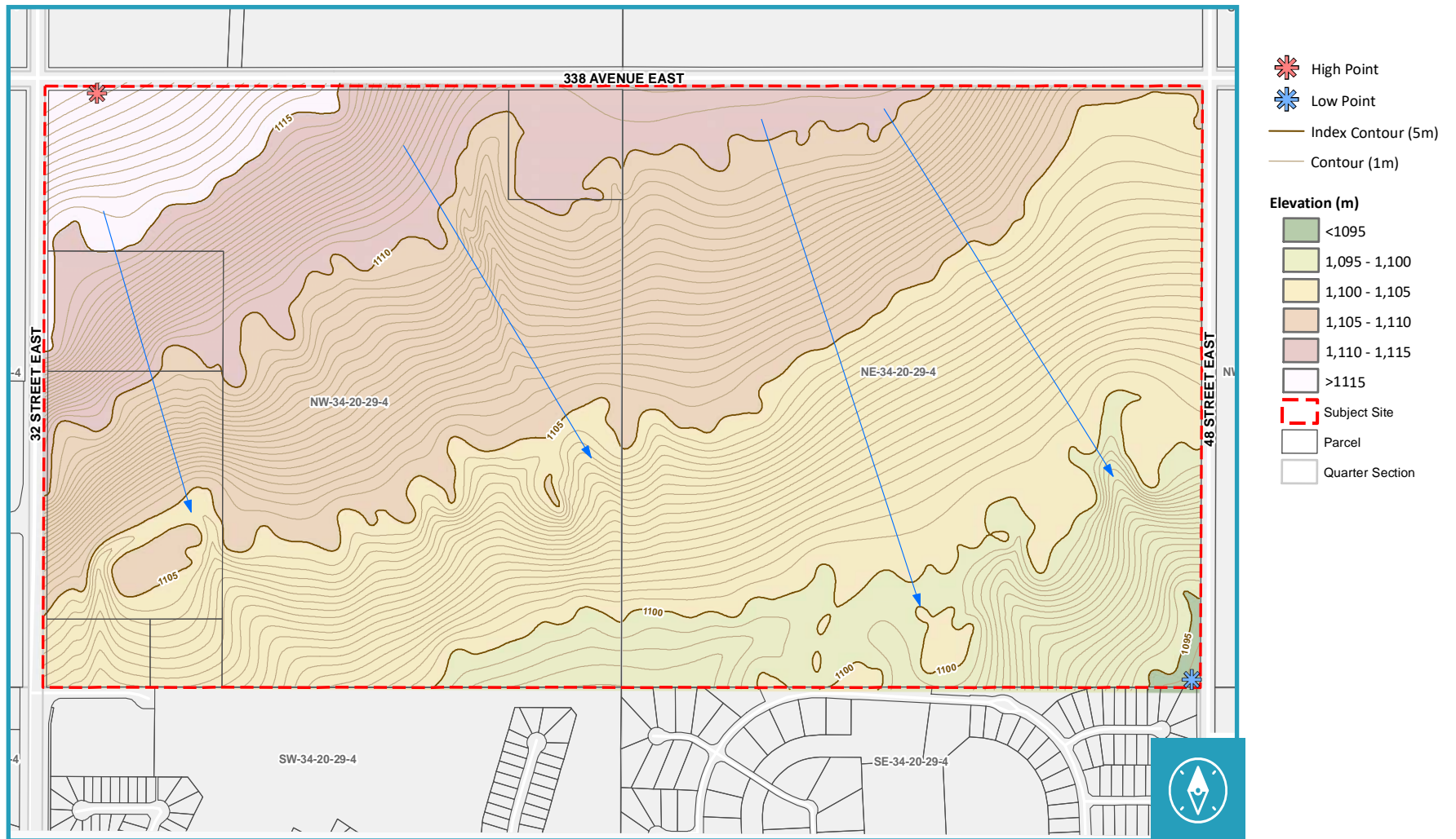
Figure 7 | Topography
